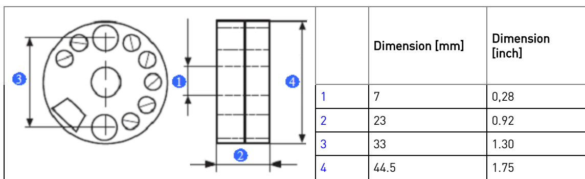
Figure 20: C520 dimensions
