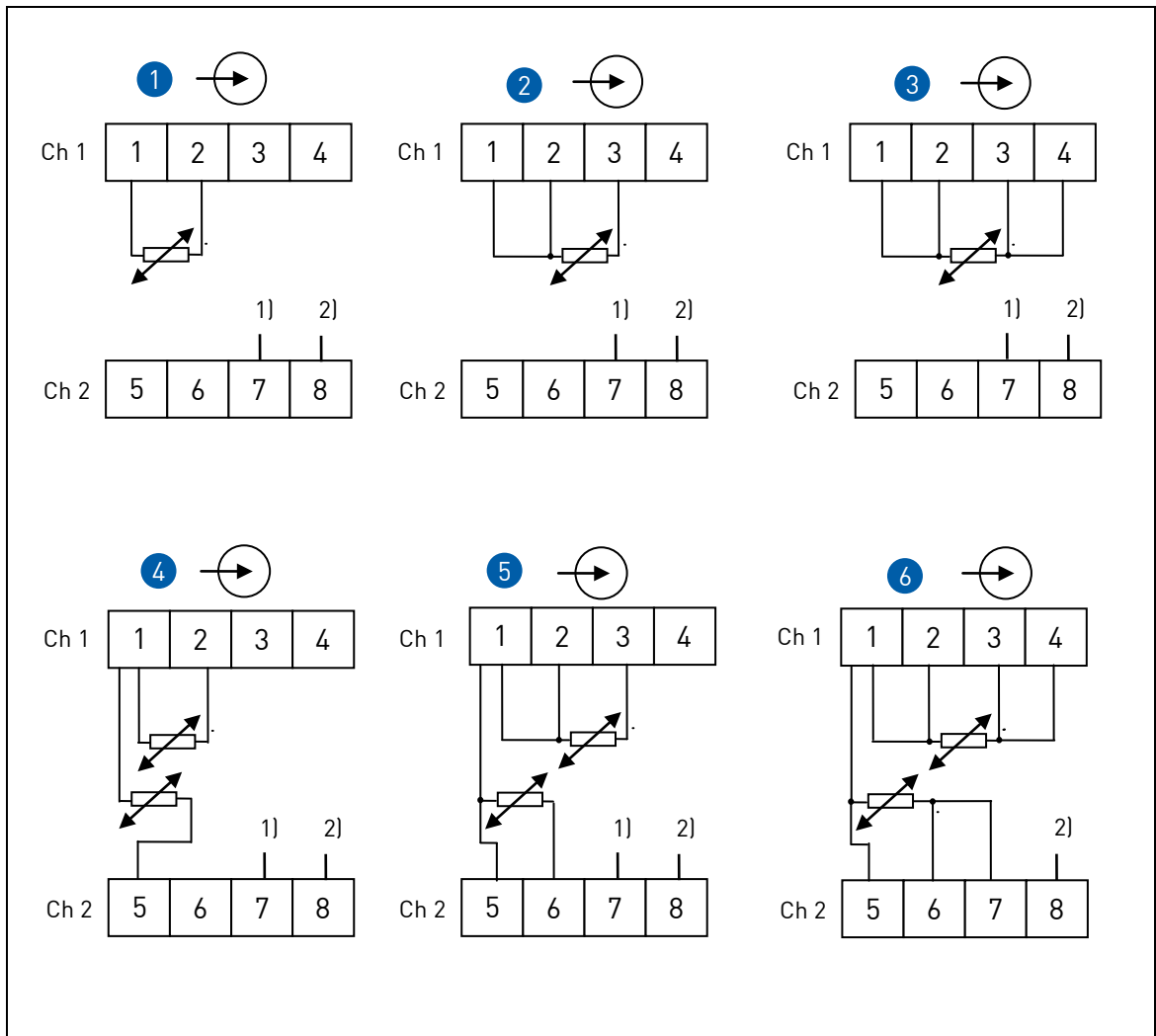
Figure 9: Installation diagram, RTD connections for R520/R520X
