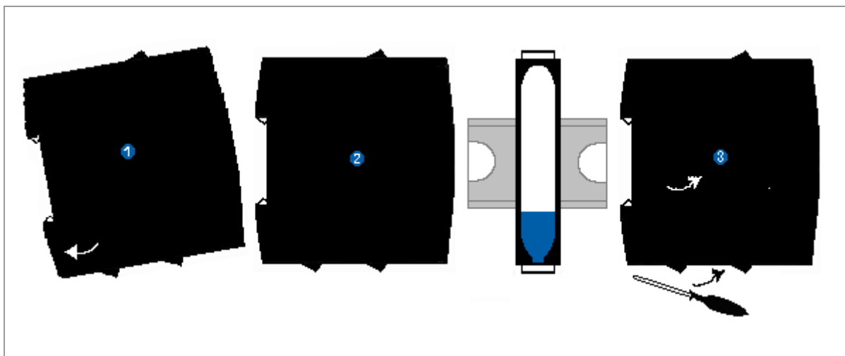
Figure 4: Rail installation
