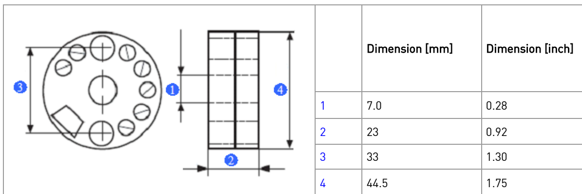
Figure 22: C520X dimensions
