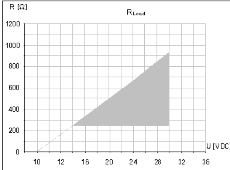
Figure 21: C520X output load diagram
