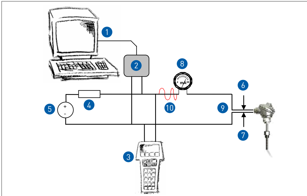
Figure 15: C520 point-to-point analog / digital mode
