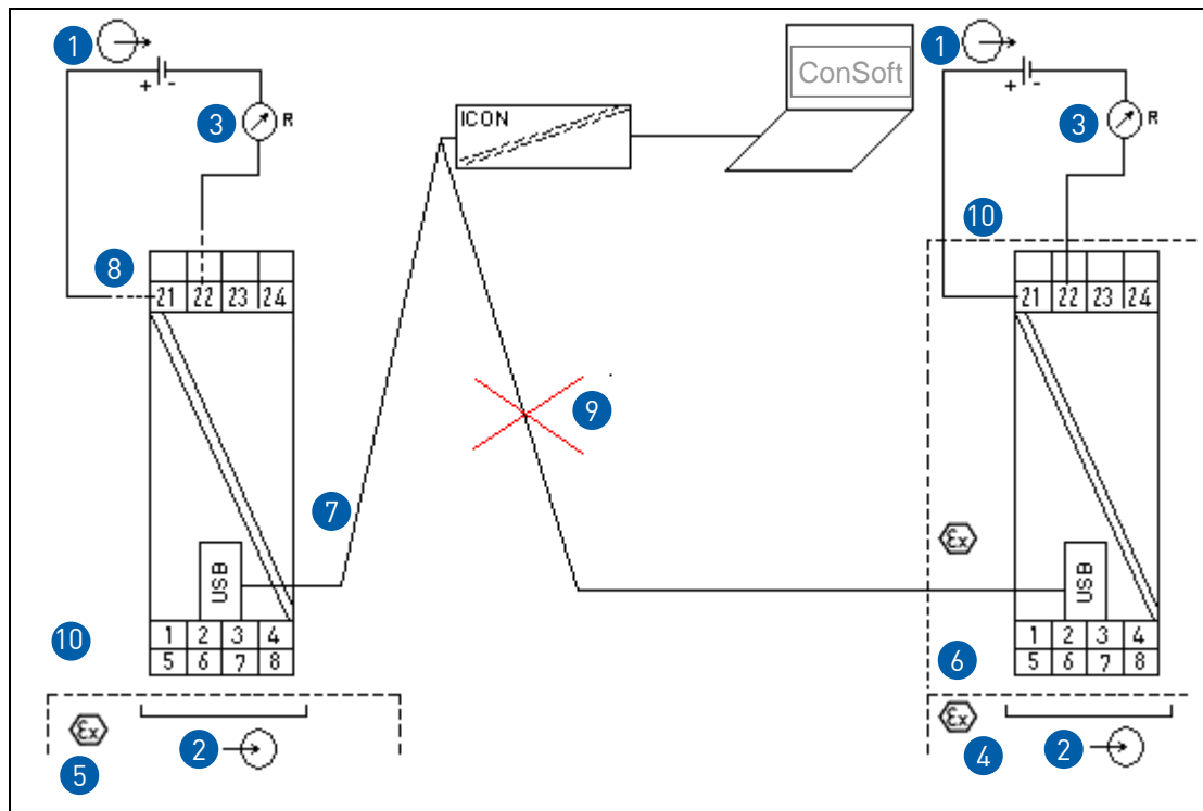
Figure 18: R520X connection to USB Interface and ConSoft during configuration
