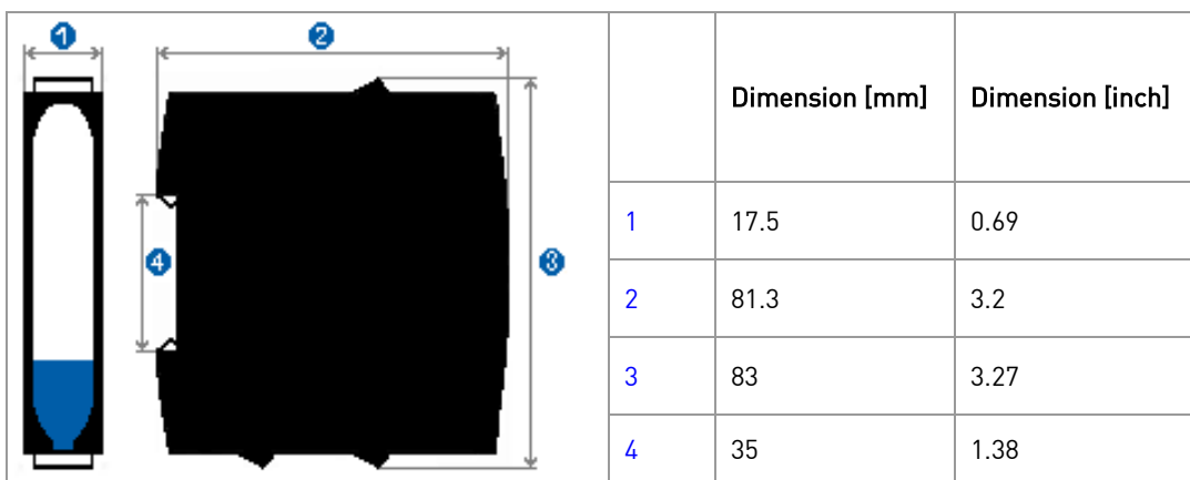
Figure 26: R520X dimensions
