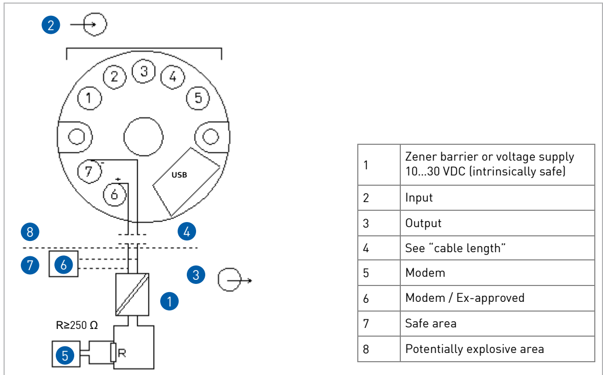
Figure 8: C520X connection
