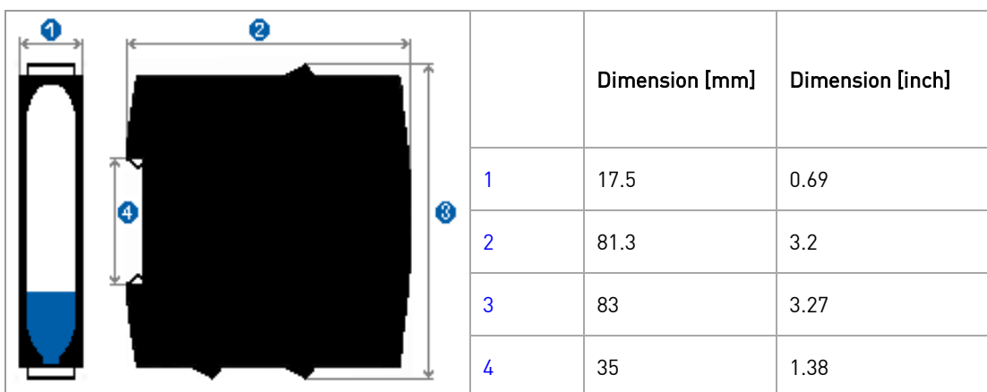
Figure 24: R520 dimensions
